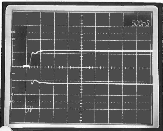
5 V/DIV, 500 NS/DIV R_L \approx 3 \Omega (RISE TIME)
